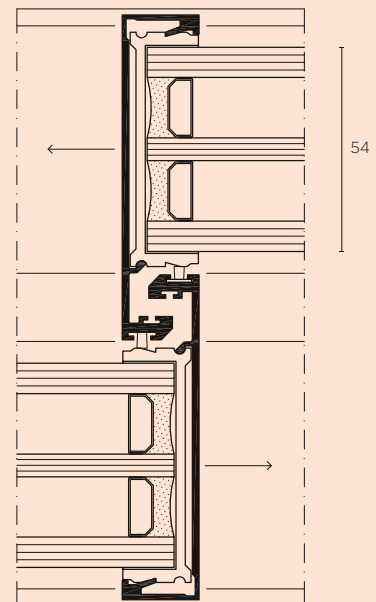
Sky-Frame 3 (Glas 54 mm)
